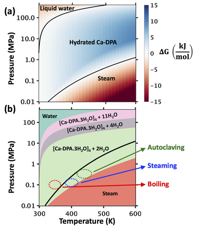
FIG. 7. (a) Free energy difference of water and hydrated Ca-DPA for different temperatures and pressures has distinct regions of hydration and dehydration. (b) Regions of stability correspond to various hydrations in Ca-DPA. The solid black line is the liquid-vapor boundary of water.
