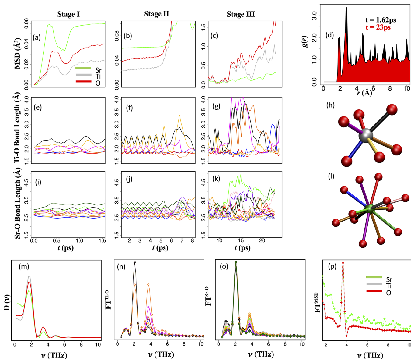
Figure 2. Lattice motion. (a–c) Atomic mean square displacement (MSD) for Sr (green), Ti (gray), and O (red) atoms divided into three stages of motion. Stage I is marked by the gradual activation of low-frequency phonons. Stage II is marked by a high-frequency MSD drift, indicating the activation of higher frequency phonon modes. Stage III is marked by lattice destabilization and amorphization driven by Ti and O diffusion. (d) Radial distribution function g(r) at time t = 1.62 and 23 ps as it begins to amorphize. (e–g) Time evolution of Ti–O bond lengths for a given Ti atom divided into the three stages of motion, with specific Ti–O bonds colored in panel h. Similarly, panels i–k show the Sr–O bond evolution for a selected Sr atom with specific bonds colored in panel l. (m–p) Fourier transforms of the velocity autocorrelation function (m), average Ti–O bond lengths for each bond type (n), average Sr–O bond lengths for each bond-type (o), and MSD during Stage II of motion (p). These Fourier transforms indicate two dominant phonon frequencies, \sim 1.8 and \sim 3.8 THz.
