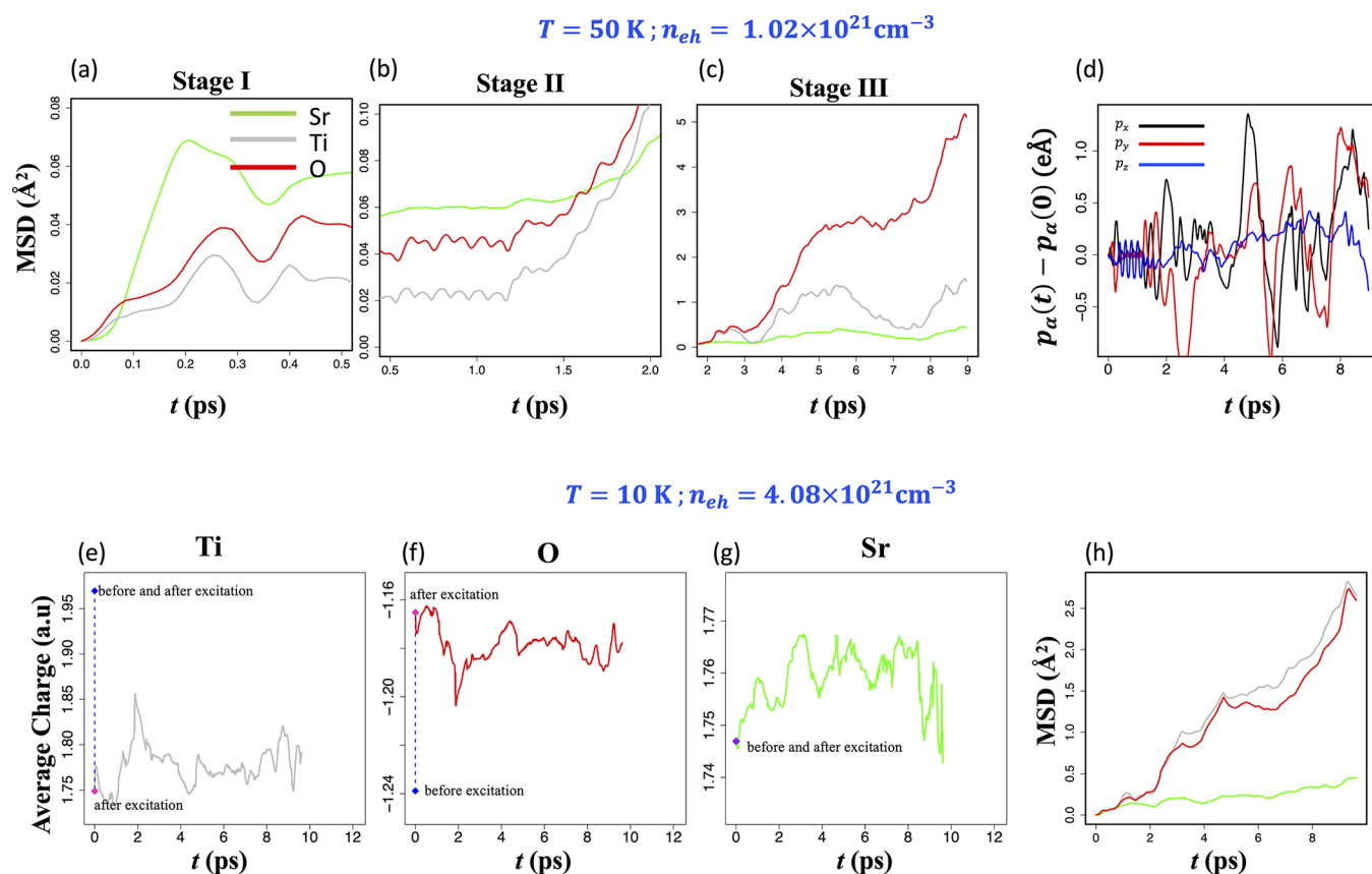
Figure 4. Effect of temperature and carrier concentration. (a–c) Atomic MSD at 50 K divided into three stages, as at 10 K, but the resonance period is now much shorter. (d) Time evolution of the classical PBC-compliant dipole moment. At 50 K, more phonon modes are activated, which leads to an earlier onset of violent fluctuations in the classical PBC-compliant dipole moment, leading to faster lattice destabilization. (e–g) Average charge dynamics for Ti, O, and Sr at 10 K with an increased carrier concentration. The increased carrier concentration leads to a large charge transfer from O–Ti, which immediately destabilizes the lattice, resulting in Ti and O diffusion, which is shown in panel h.
