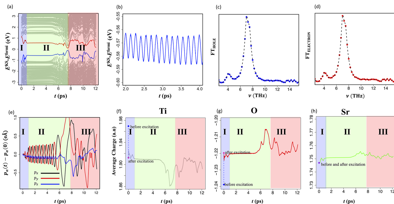
Figure 3. Electron–hole and charge dynamics. (a) Time evolution of Kohn–Sham (KS) eigenvalues from 0 to 12 ps divided into the three stages of lattice motion. (b) Zoom-in on the coherent evolution of the hole wave function during Stage II of lattice motion. (c,d) Fourier transforms of the hole and electron eigenenergy evolutions, respectively, during Stage II of motion. They both are characterized by a dominant high frequency of \sim 7.5 THz. (e) Time evolution of the classical dipole moment, as defined in eq 1. The increasing oscillations of the classical dipole are indicative of an unstable polarization buildup during the coherent motion period. (f–h) Dynamics of the average charge for Ti, O, and Sr, respectively. There is an initial charge transfer from O–Ti as a result of excitation followed by a period of equilibration as the charge dynamics attempt to stabilize. The unstable polarization buildup ultimately destabilizes the charge dynamics, resulting in a large charge transfer from O–Ti as the lattice destabilizes.
