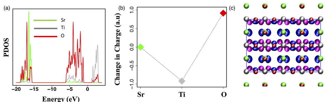
Figure 1. Initial excitation. (a) Atom-projected partial density of states (PDOS) in STO. The valence band maximum (VBM) is primarily composed of O states, whereas the conduction band minimum (CBM) is primarily composed of Ti states, indicating O-to-Ti charge transfer upon excitation. (b) Total change in charge of each atom type after excitation. (c) (010) projection of electron (magenta) and hole (blue) wave functions for excitation from VBM to CBM, where Sr, Ti, and O atoms are colored in green, gray, and red, respectively. As expected, the electron and hole wave functions are centered on Ti and O atoms, respectively.
